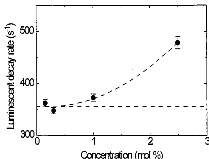
Fig. 4. Luminescent decay rate vs concentration of \text{Ni}^{2+} in \text{BaLiF}_3 at room temperature.
